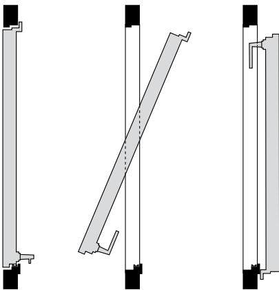
Locking position
