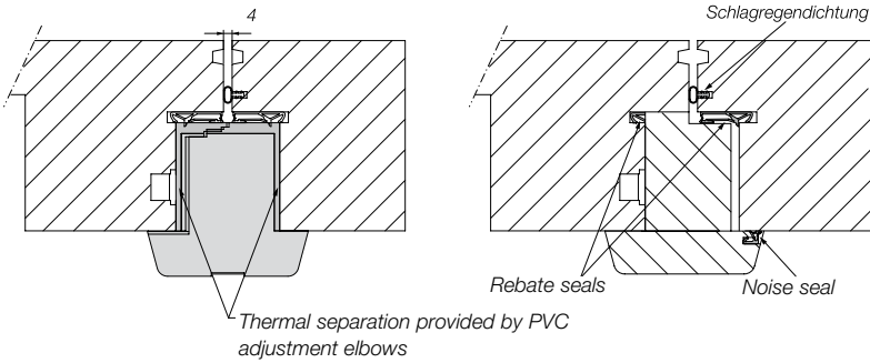
Section above the pivot hinge (three sealing levels)
