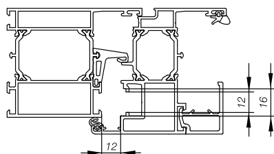
Vertical section KSP on the timber window
