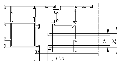
Vertical section KSP on the aluminium window
