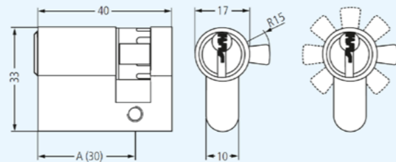
Winkhaus Enkel profil/euro cylinder Key One XPERT.
